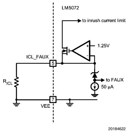
FIGURE 7. Input Inrush Limit Programming via R_{ICL}
