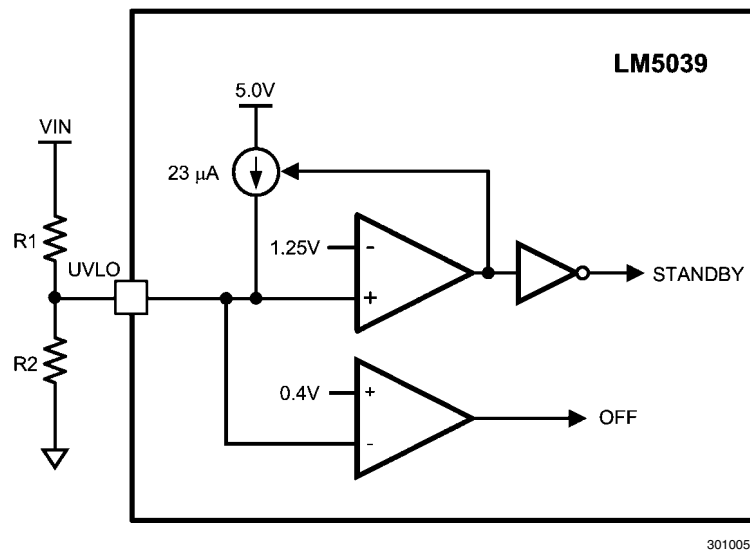
FIGURE 10. Basic UVLO Configuration
