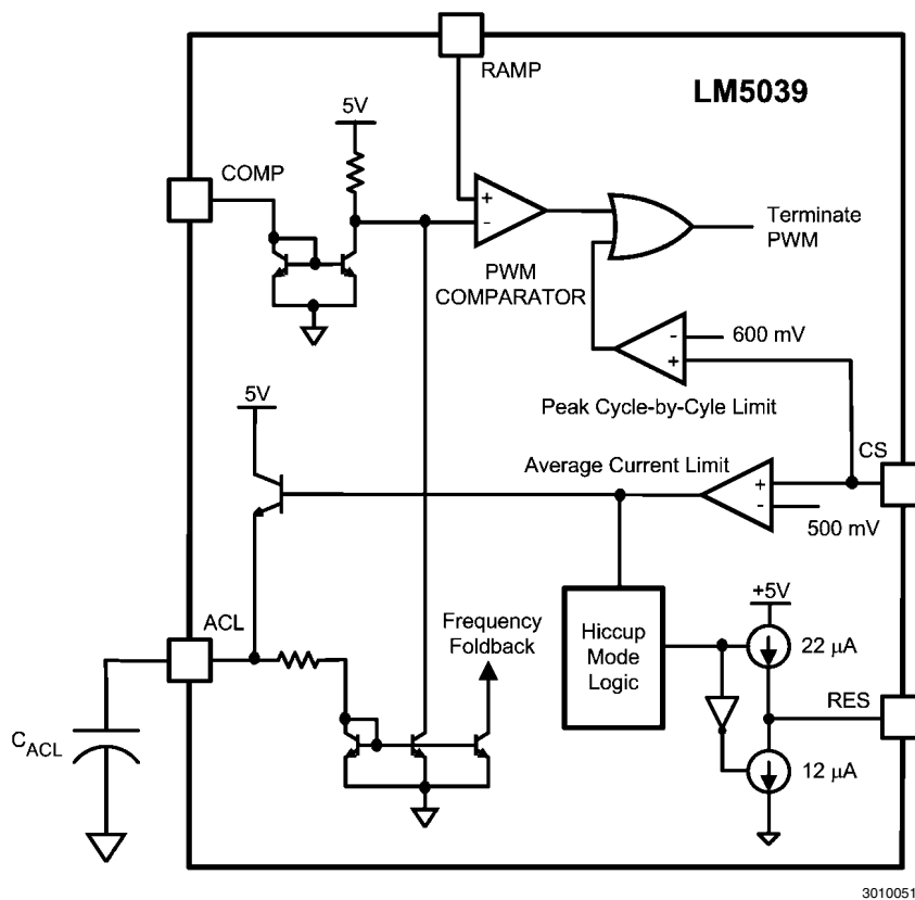
FIGURE 2. Peak Cycle-by-Cycle and Average Current Limit Circuitry
