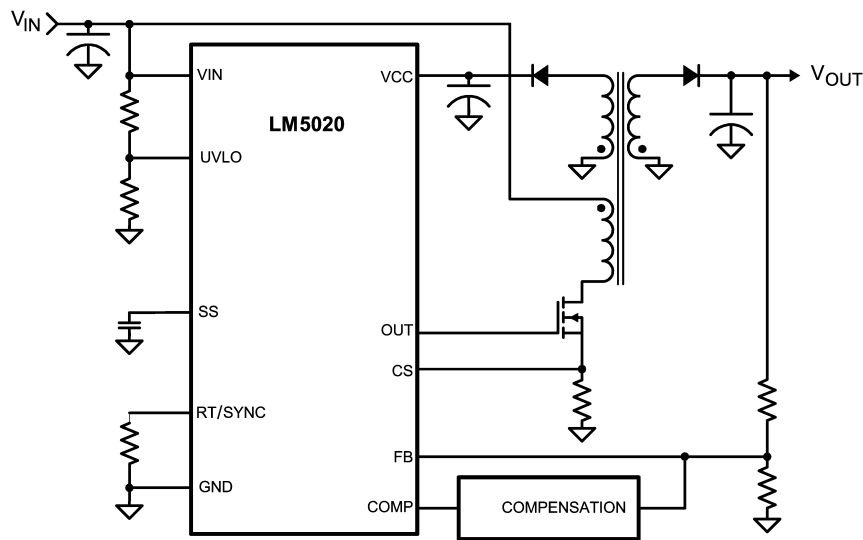
Non-Isolated Flyback Converter
