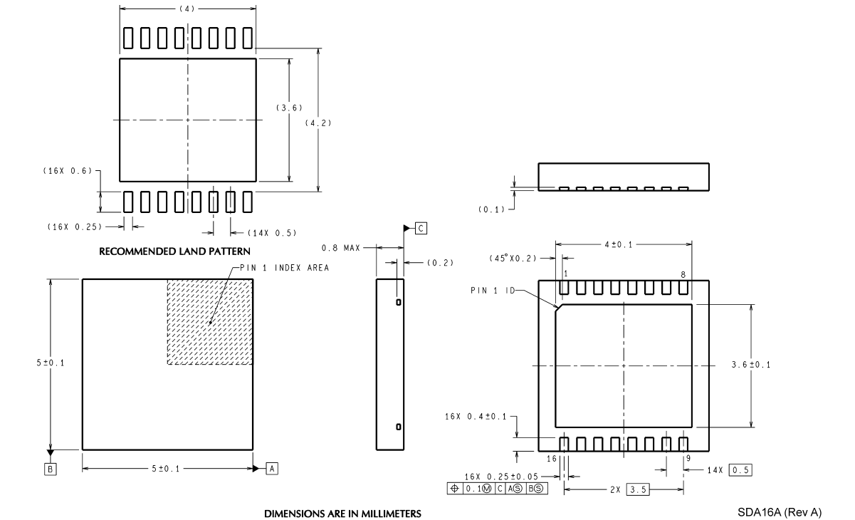
16-Lead LLP Surface Mount Package NS Package Number SDA16A
