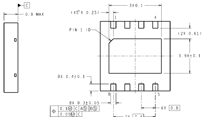
8-Lead LLP Package NS Package Number SDC08B
