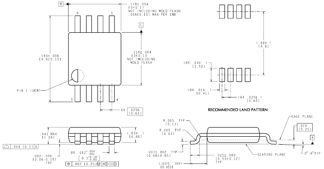
8-Lead MSOP Package NS Package Number MUA08A
