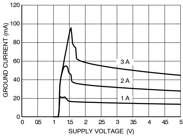
Figure 12. Ground Current vs. Supply Voltage (1.24 V)
