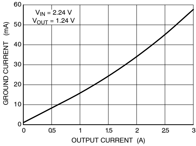
Figure 10. Ground Current vs. Output Current
