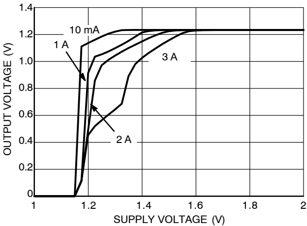
Figure 8. Dropout Characteristics (1.24 V)
