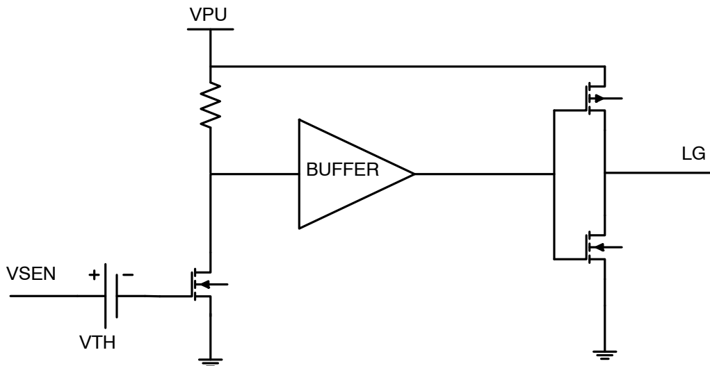
Figure 4. PreOVP circuit
