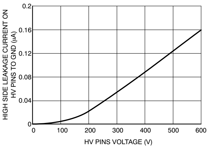
Figure 38. Leakage Current on High Voltage Pins (600 V) to Ground vs. V BRIDGE Voltage (V BRIDGE = V BOOT = V DRV_HI )
