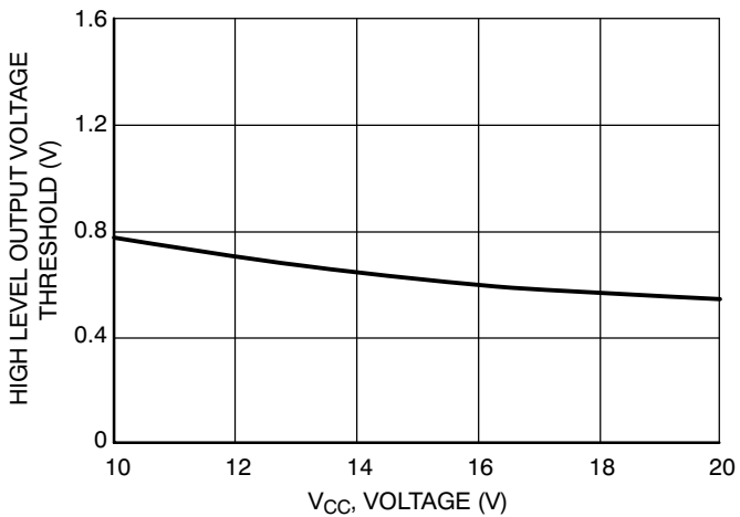
Figure 32. High Level Output Voltage vs. Supply Voltage ( V_{CC} = V_{BOOT} )
