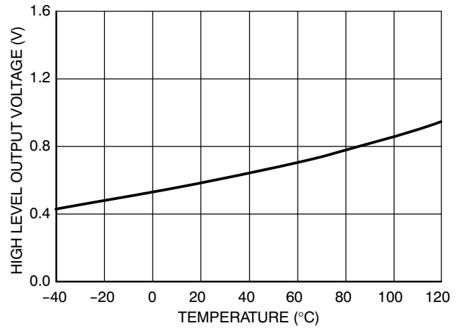
Figure 33. High Level Output Voltage vs. Temperature
