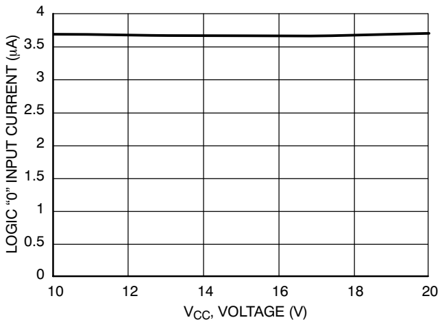
Figure 26. Logic "0" Input Current vs. Supply Voltage ( V_{CC} = V_{BOOT} )
