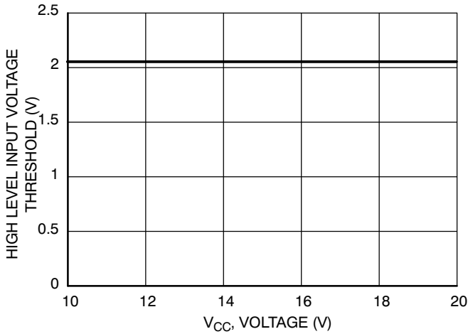
Figure 24. High Level Input Voltage Threshold vs. Supply Voltage ( V_{CC} = V_{BOOT} )
