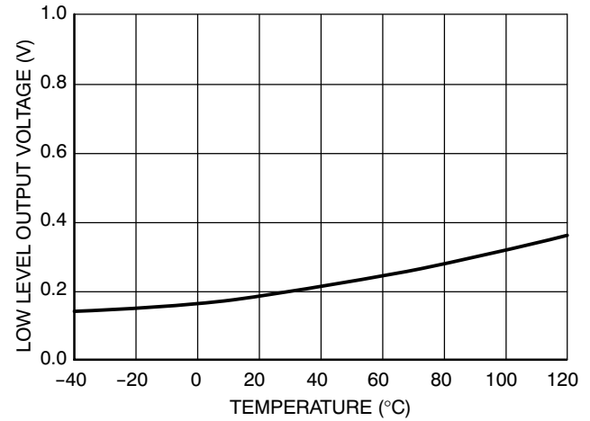
Figure 31. Low Level Output Voltage vs. Temperature
