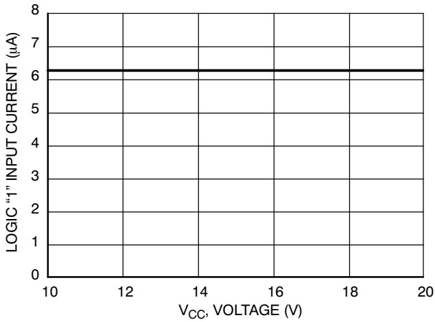
Figure 28. Logic "1" Input Current vs. Supply Voltage ( V_{CC} = V_{BOOT} )
