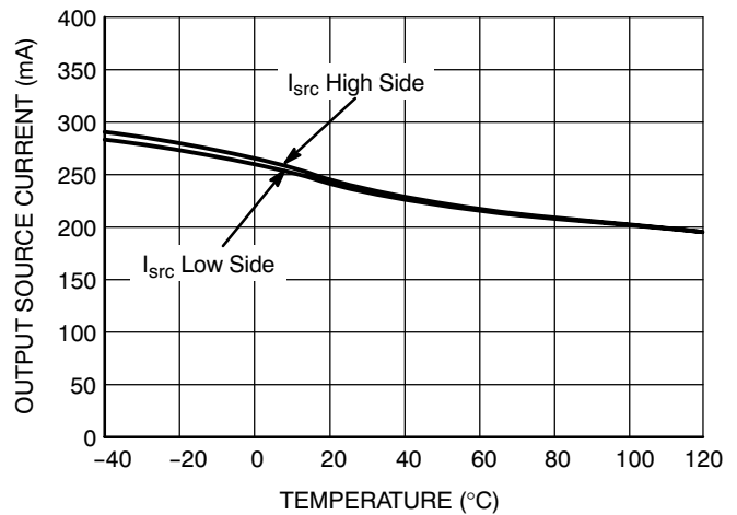
Figure 35. Output Source Current vs. Temperature
