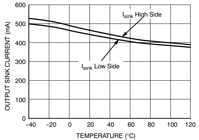
Figure 37. Output Sink Current vs. Temperature
