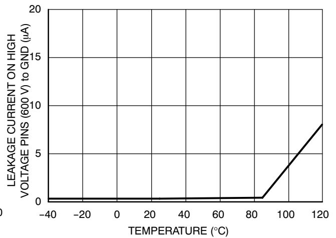
Figure 39. Leakage Current on High Voltage Pins (600 V) to Ground vs. Temperature (V BRIDGE = V BOOT = V DRV_HI = 600 V)
