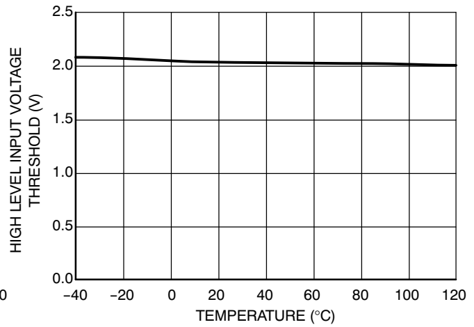
Figure 25. High Level Input Voltage Threshold vs. Temperature
