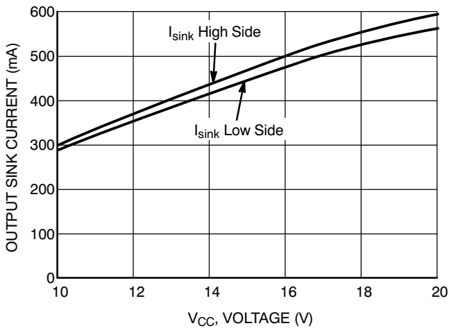
Figure 36. Output Sink Current vs. Supply Voltage (V CC = V BOOT )
