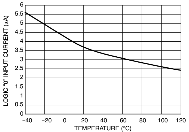
Figure 27. Logic "0" Input Current vs. Temperature
