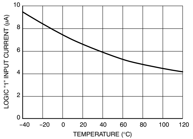
Figure 29. Logic "1" Input Current vs. Temperature
