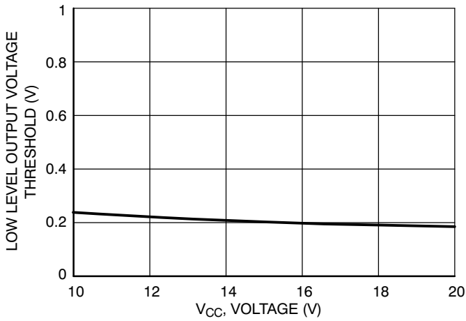
Figure 30. Low Level Output Voltage vs. Supply Voltage ( V_{CC} = V_{BOOT} )
