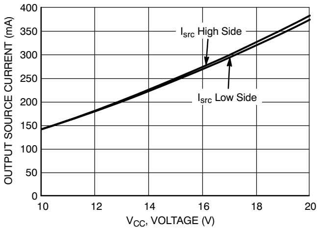
Figure 34. Output Source Current vs. Supply Voltage (V CC = V BOOT )
