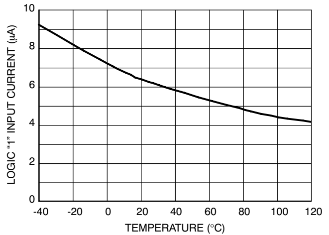
Figure 25. Logic "1" Input Current vs. Temperature
