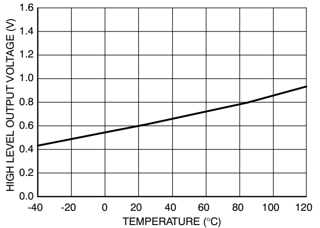
Figure 29. High Level Output Voltage vs. Temperature
