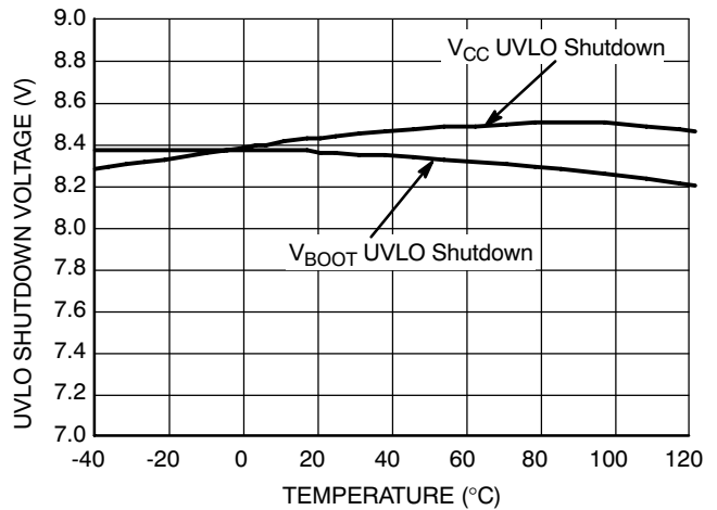
Figure 41. UVLO Shutdown Voltage vs. Temperature
