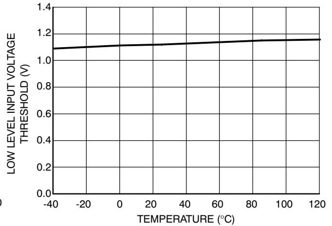
Figure 19. Low Level Input Voltage Threshold vs. Temperature
