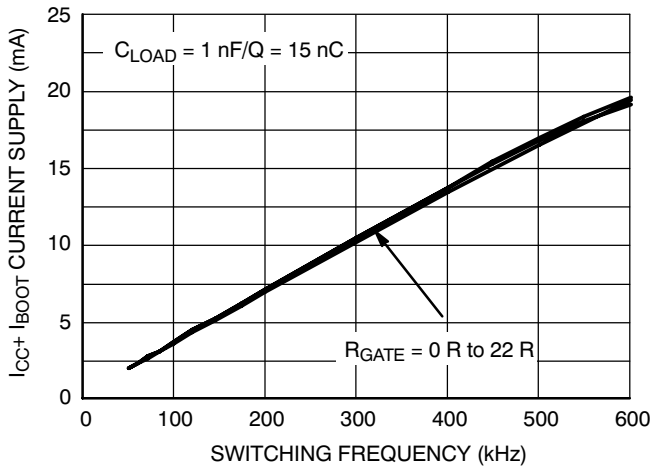
Figure 42. I_{CC1} Consumption vs. Switching Frequency with 15 nC Load on Each Driver @ V_{CC} = 15 V
