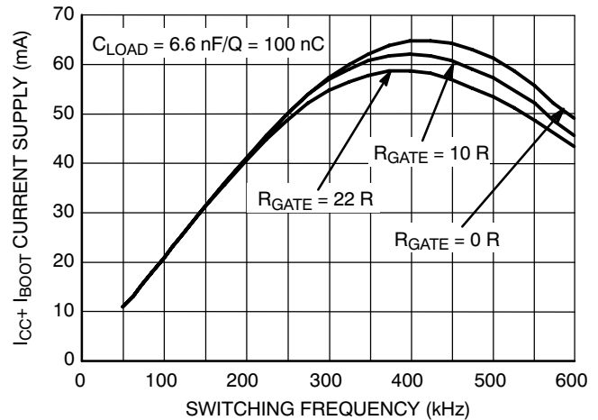
Figure 45. I_{CC1} Consumption vs. Switching Frequency with 100 nC Load on Each Driver @ V_{CC} = 15 V
