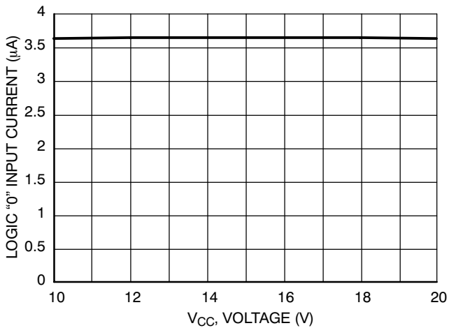
Figure 22. Logic "0" Input Current vs. Supply Voltage ( V_{CC} = V_{BOOT} )
