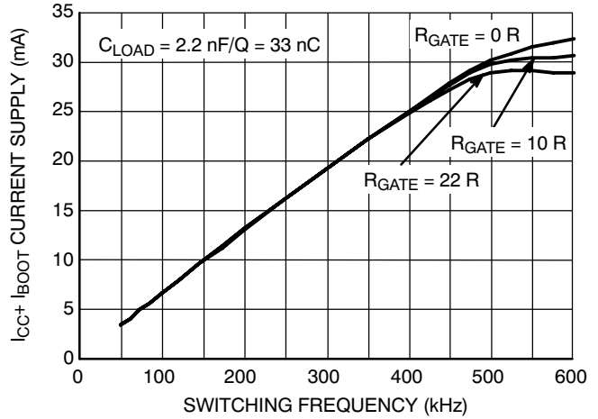
Figure 43. I_{CC1} Consumption vs. Switching Frequency with 33 nC Load on Each Driver @ V_{CC} = 15 V
