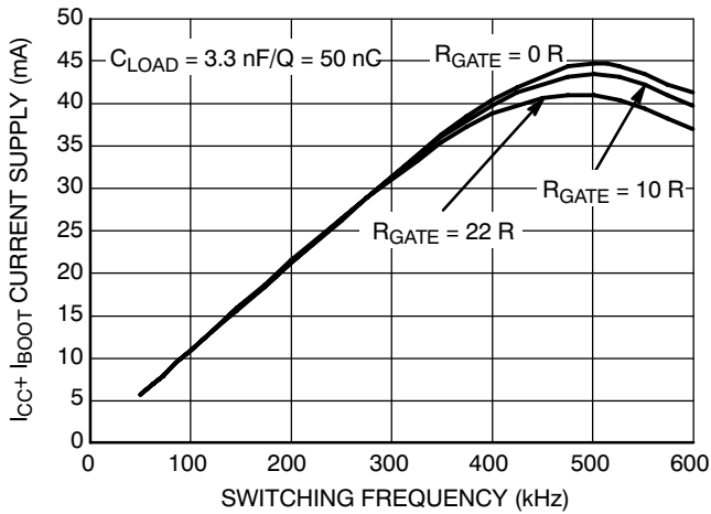
Figure 44. I_{CC1} Consumption vs. Switching Frequency with 50 nC Load on Each Driver @ V_{CC} = 15 V
