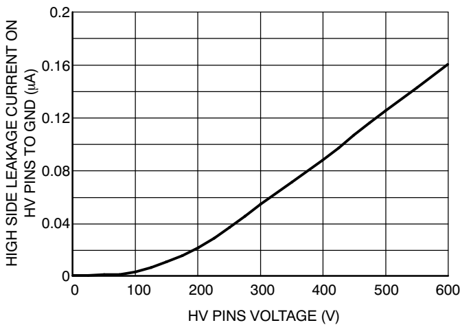
Figure 34. Leakage Current on High Voltage Pins (600 V) to Ground vs. V BRIDGE Voltage (V BRIDGE = V BOOT = V DRV_HI )
