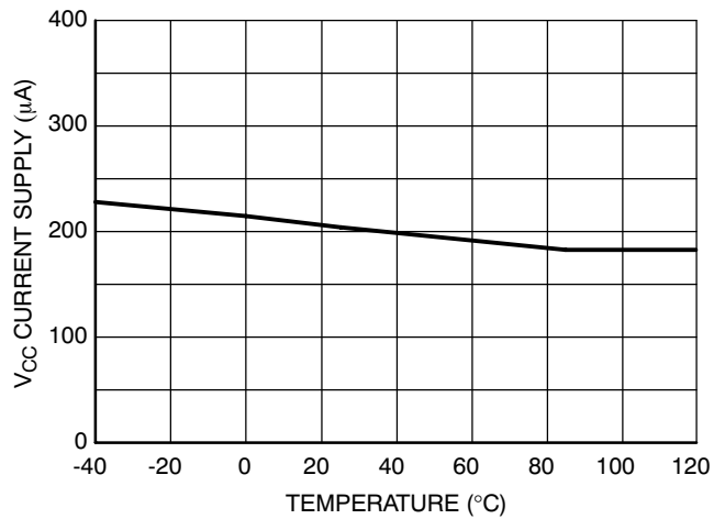
Figure 39. V_{CC} Supply Current vs. Temperature
