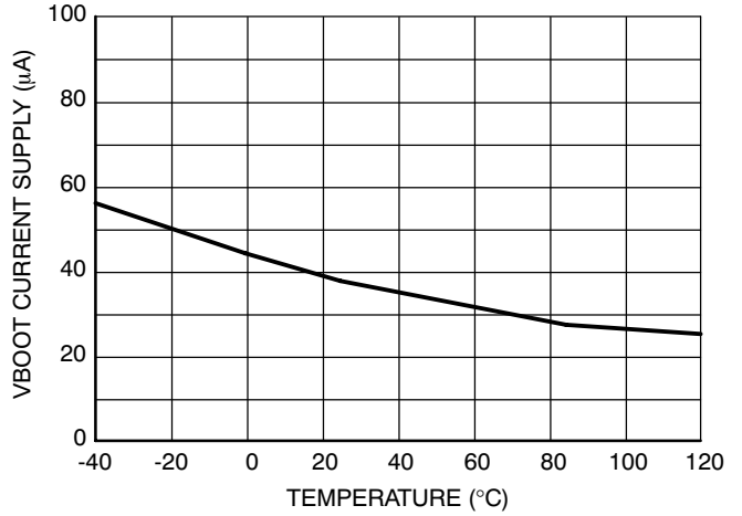
Figure 37. V_{BOOT} Supply Current vs. Temperature
