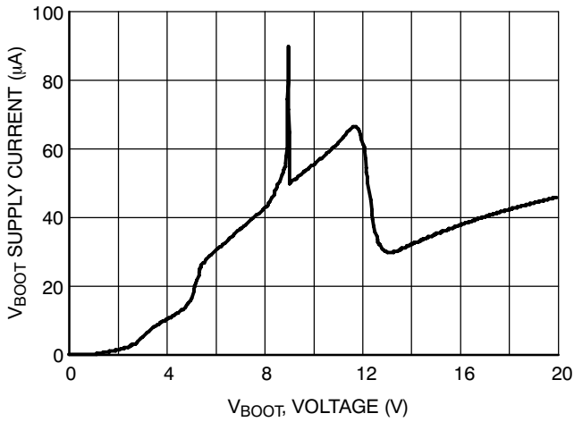
Figure 36. V_{BOOT} Supply Current vs. Bootstrap Supply Voltage
