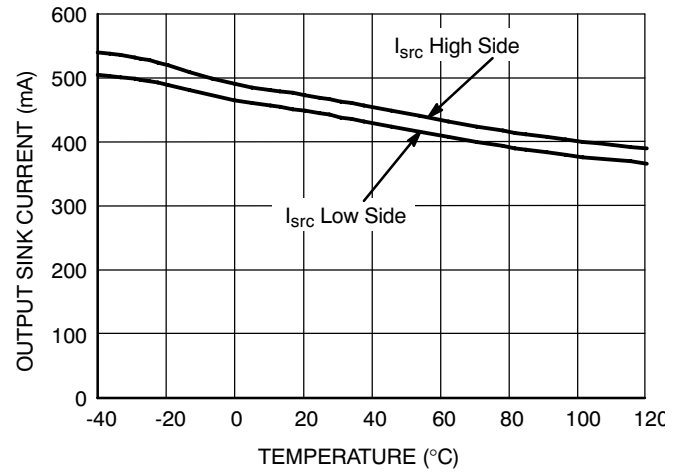
Figure 33. Output Sink Current vs. Temperature
