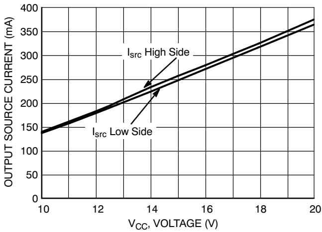
Figure 30. Output Source Current vs. Supply Voltage (V CC = V BOOT )
