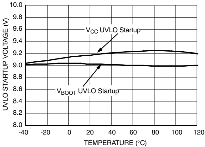
Figure 40. UVLO Startup Voltage vs. Temperature
