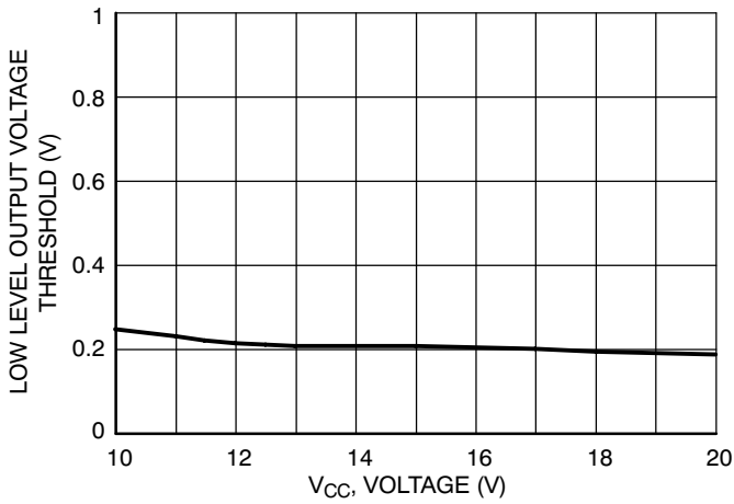
Figure 26. Low Level Output Voltage vs. Supply Voltage ( V_{CC} = V_{BOOT} )
