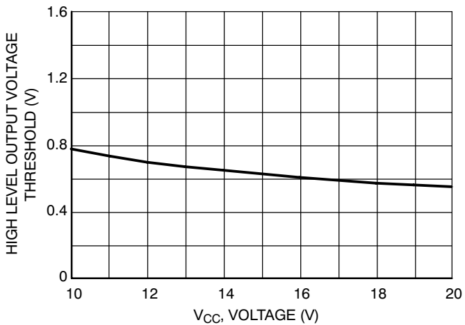
Figure 28. High Level Output Voltage vs. Supply Voltage ( V_{CC} = V_{BOOT} )
