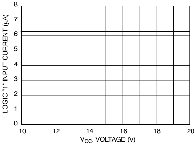
Figure 24. Logic "1" Input Current vs. Supply Voltage ( V_{CC} = V_{BOOT} )
