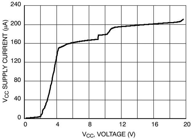
Figure 38. V_{CC} Supply Current vs. V_{CC} Supply Voltage
