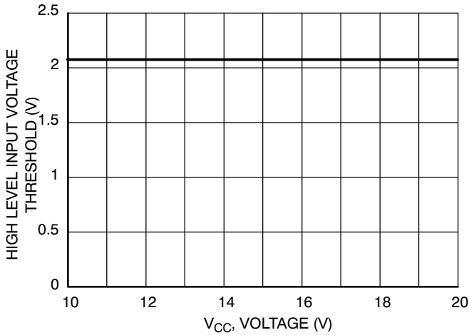
Figure 20. High Level Input Voltage Threshold vs. Supply Voltage ( V_{CC} = V_{BOOT} )
