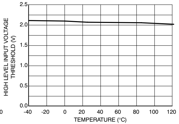
Figure 21. High Level Input Voltage Threshold vs. Temperature
