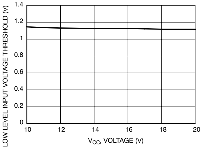
Figure 18. Low Level Input Voltage Threshold vs. Supply Voltage ( V_{CC} = V_{BOOT} )
