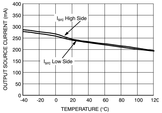
Figure 31. Output Source Current vs. Temperature
