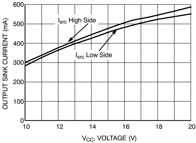
Figure 32. Output Sink Current vs. Supply Voltage (V CC = V BOOT )
