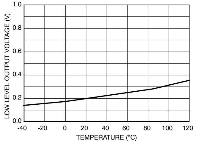
Figure 27. Low Level Output Voltage vs. Temperature
