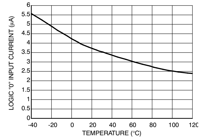
Figure 23. Logic "0" Input Current vs. Temperature
