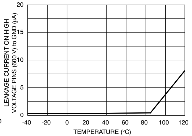
Figure 35. Leakage Current on High Voltage Pins (600 V) to Ground vs. Temperature (V BRIDGE = V BOOT = V DRV_HI = 600 V)
