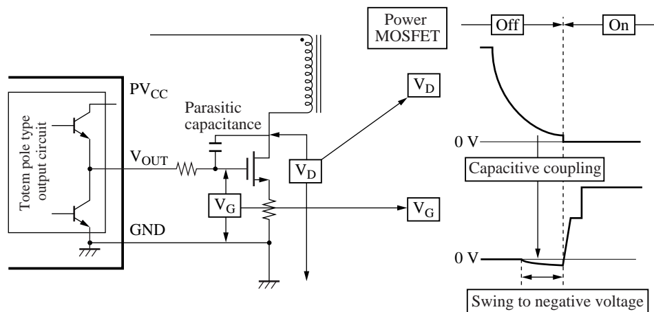
Figure 8. V_{OUT} terminal description
