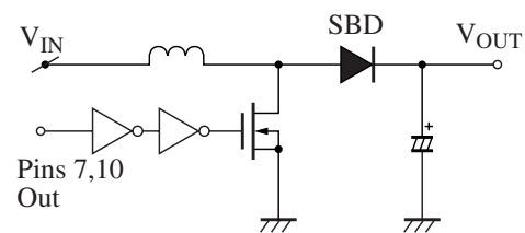
Figure 1. Output bootstrap circuit example
