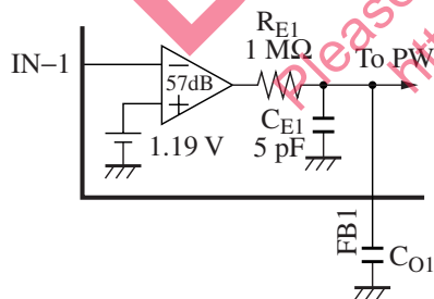
Figure 11. Error amplifier equivalent circuit
