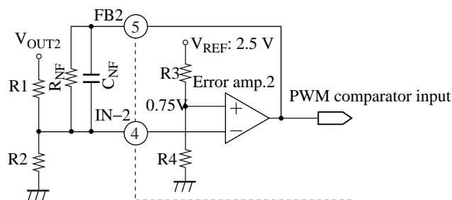
Figure 2. Connection method of error amplifier 2
