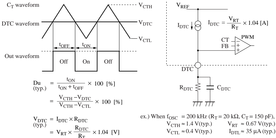
Figure 6. Dead-time setting method
