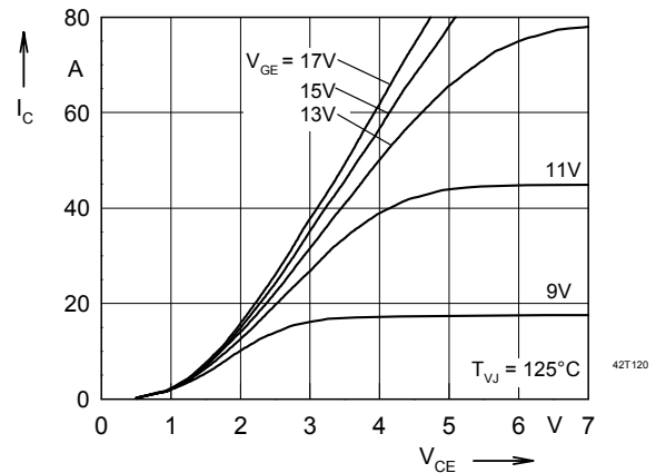
Fig. 2 Typ. output characteristics
