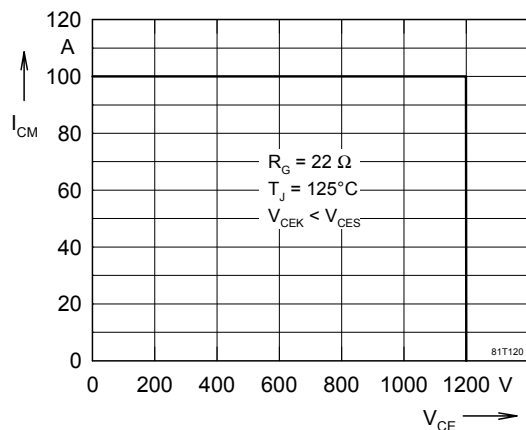
Fig. 11 Reverse biased safe operating area
