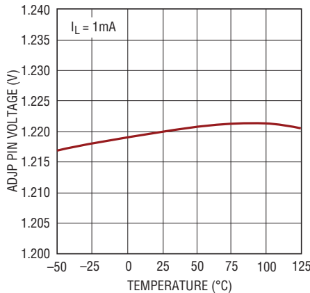
ADJP Pin Voltage
