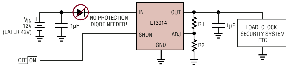
LT3014 Automotive Application
