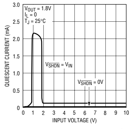
Quiescent Current
