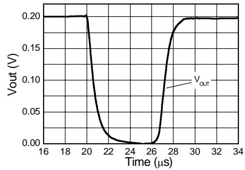
Small Sig Zero Crossing Response
