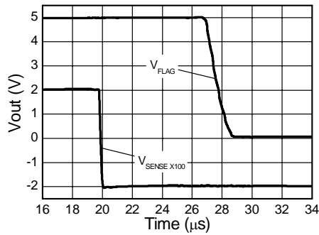
Small Sig Zero Crossing Response
