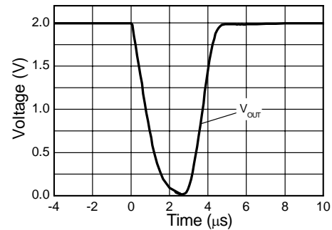
Large Sig Zero Crossing Response
