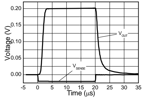
Reverse Small Signal Step Response
