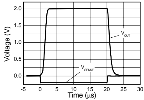
Reverse Large Signal Step Response
