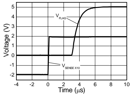
Large Sig Zero Crossing Response
