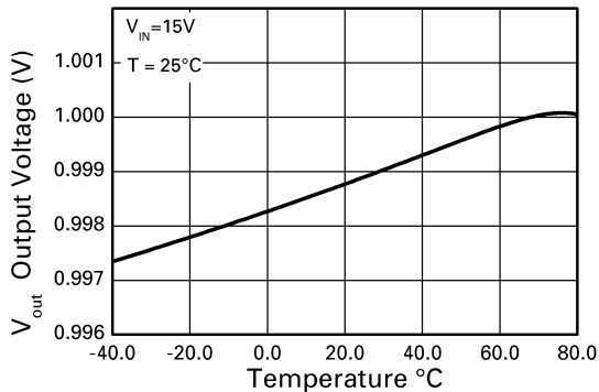
Output Voltage v Temperature
