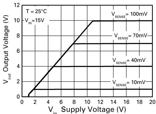
Transfer Characteristic
