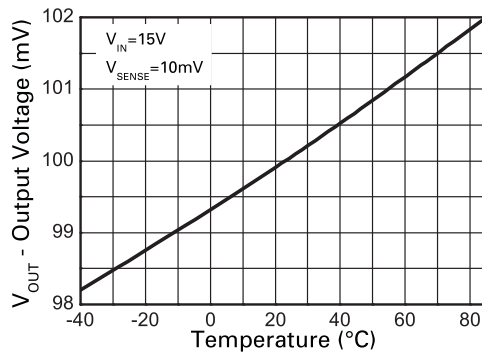
Output Voltage v Temperature
