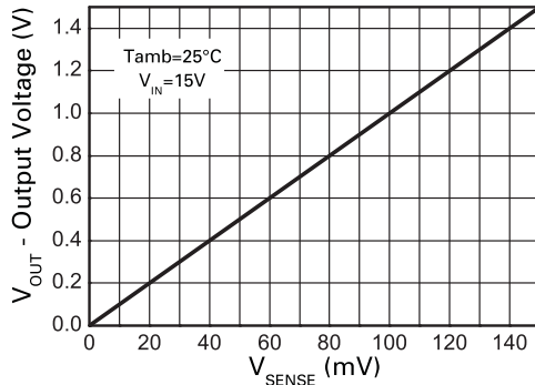
Typical Output v Sense Voltage
