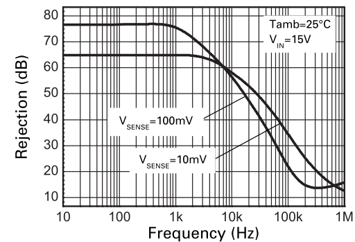
Common Mode Rejection
