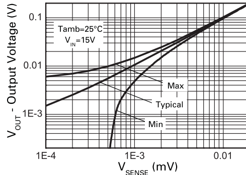
V_{OUT} v Sense Voltage
