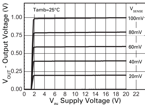
Transfer Characteristic
