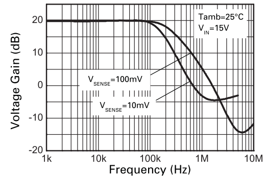
Frequency Response
