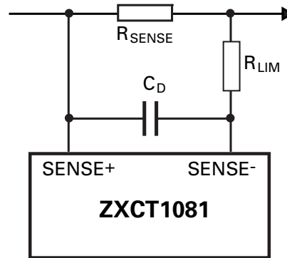
Figure 2 Protection/error sources for ZXCT1081
