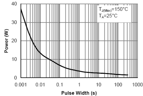
Figure 10: Single Pulse Power Rating Junction-to-Ambient (Note E)
