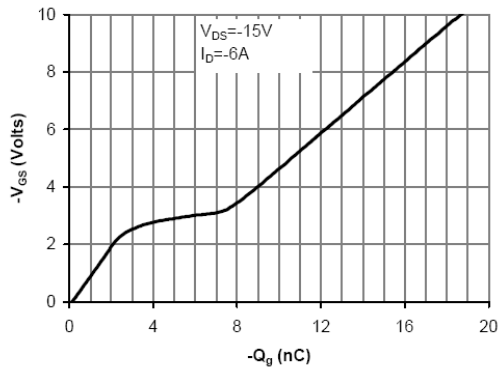
Figure 7: Gate-Charge Characteristics
