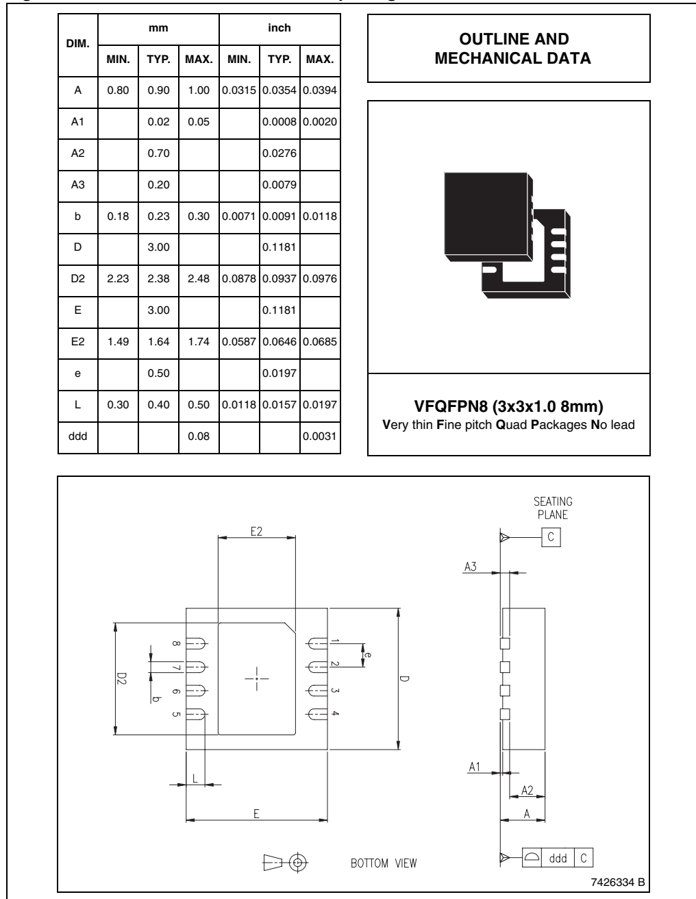
Figure 4. VFQFPN8 mechanical data &amp; package dimensions
