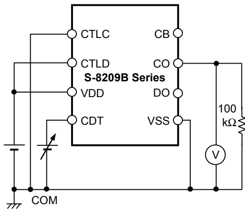
Figure 9 Test circuit 3
