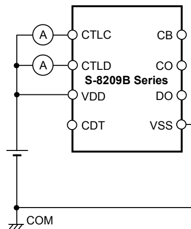
Figure 12 Test circuit 6
