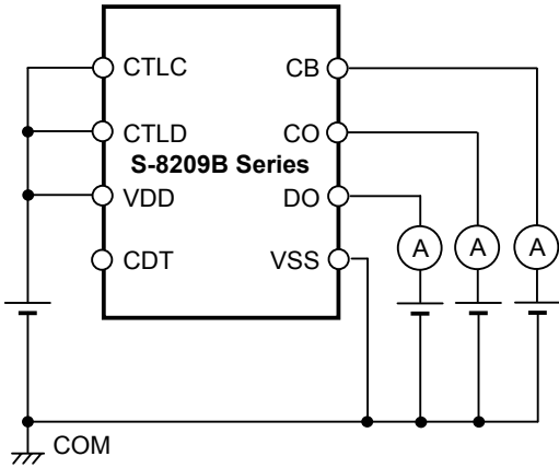
Figure 13 Test circuit 7
