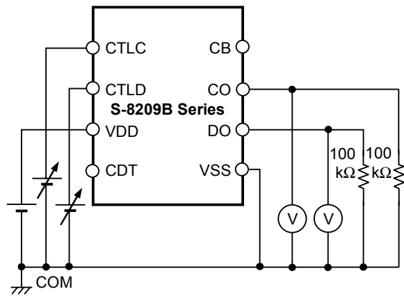
Figure 10 Test circuit 4
