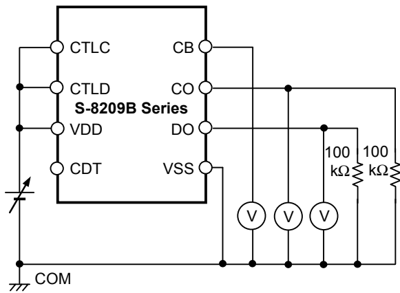
Figure 7 Test circuit 1
