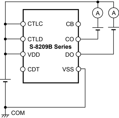
Figure 14 Test circuit 8
