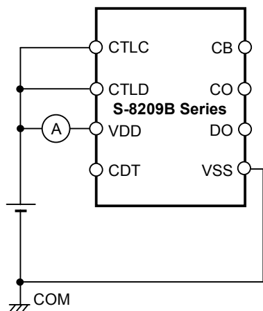
Figure 11 Test circuit 5
