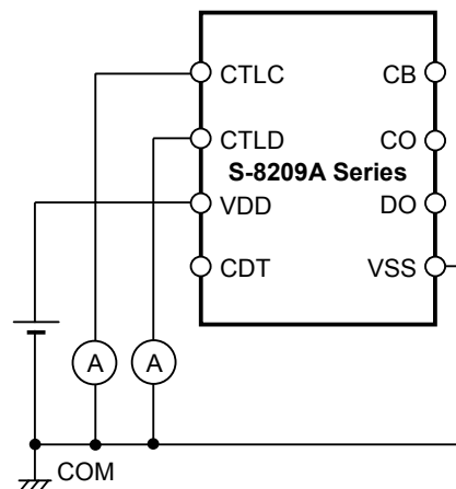
Figure 12 Test circuit 6
