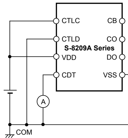
Figure 8 Test circuit 2
