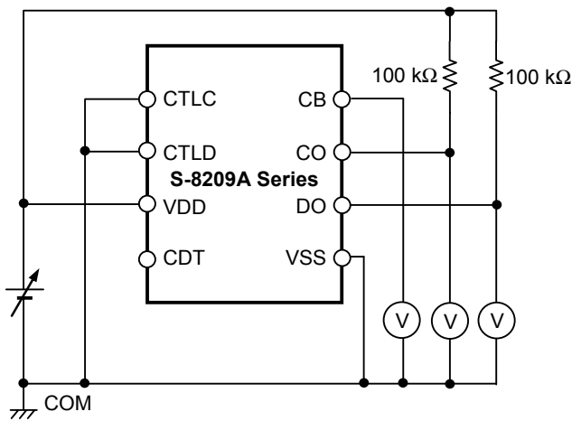
Figure 7 Test circuit 1
