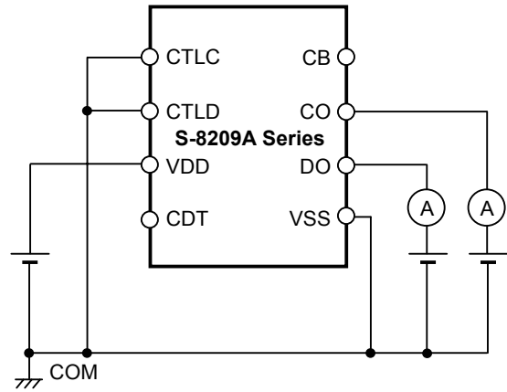
Figure 14 Test circuit 8
