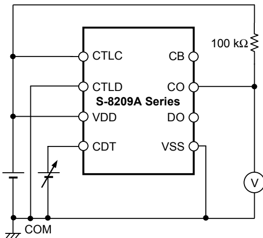
Figure 9 Test circuit 3
