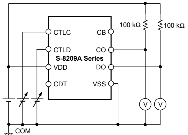
Figure 10 Test circuit 4
