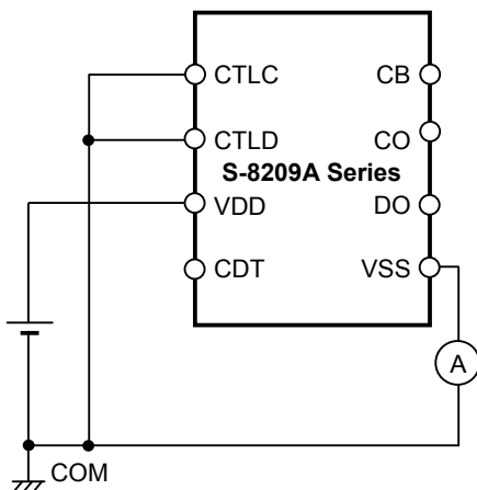
Figure 11 Test circuit 5
