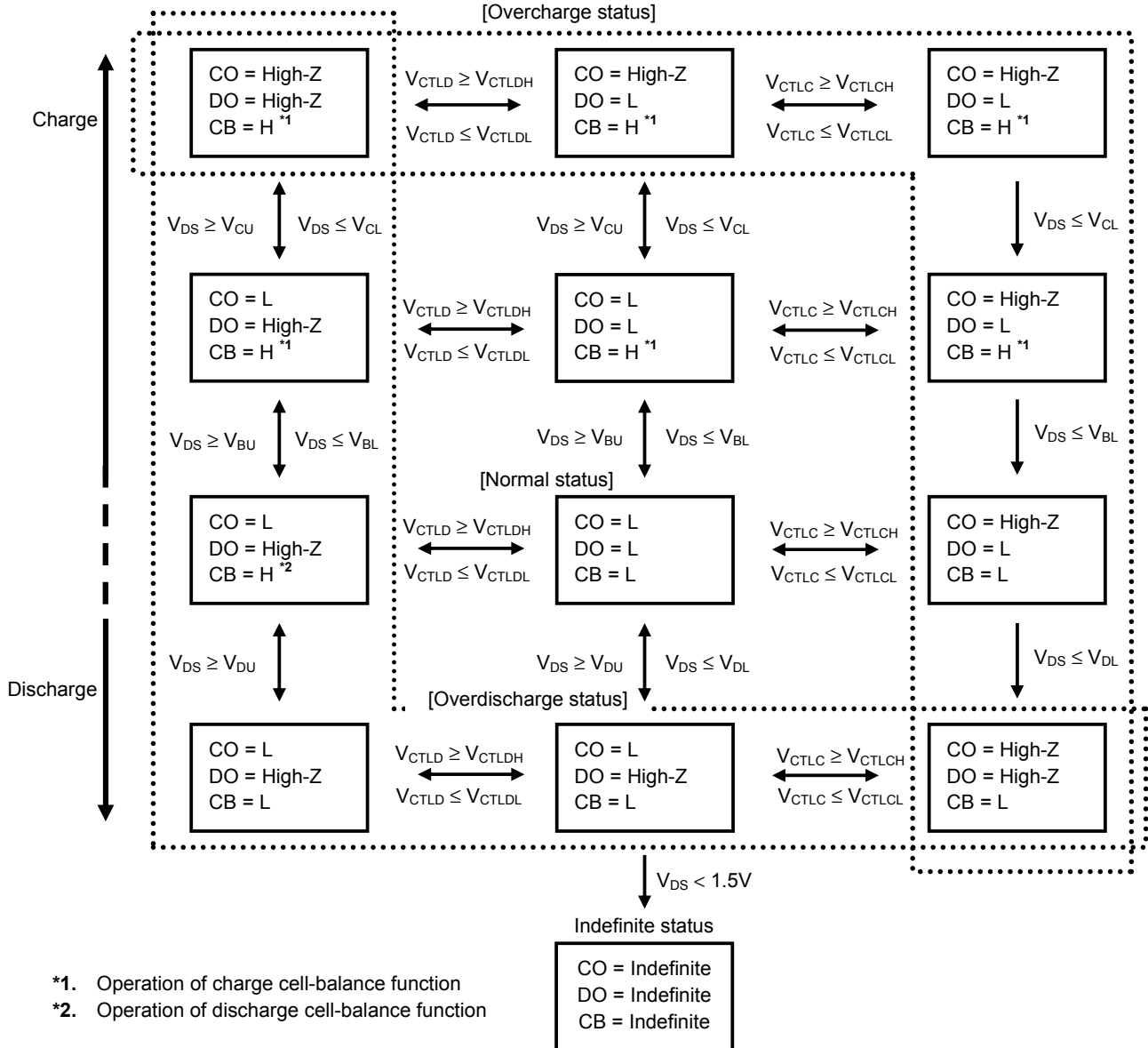
Figure 15 Operation Transition
