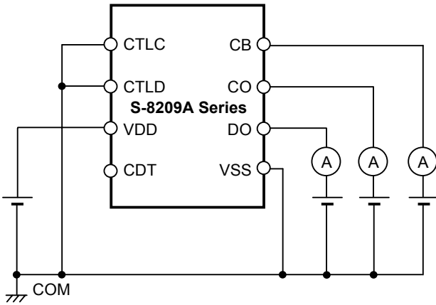
Figure 13 Test circuit 7
