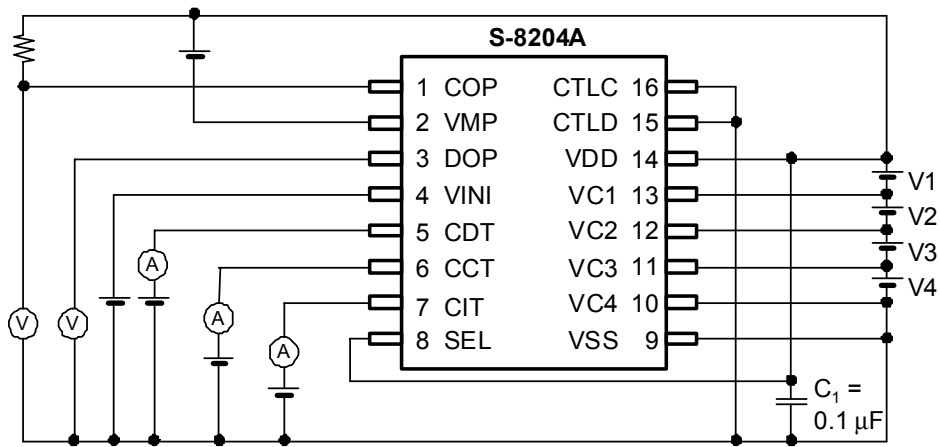
Figure 6 Test Circuit 3
