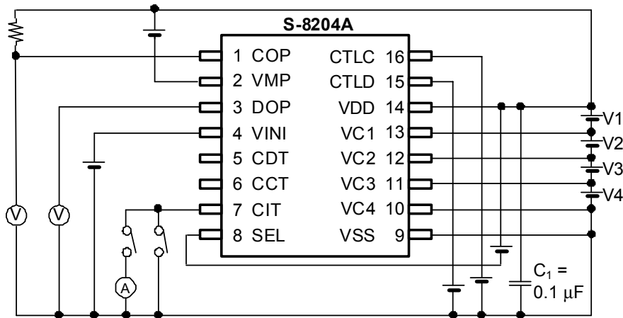
Figure 5 Test Circuit 2
