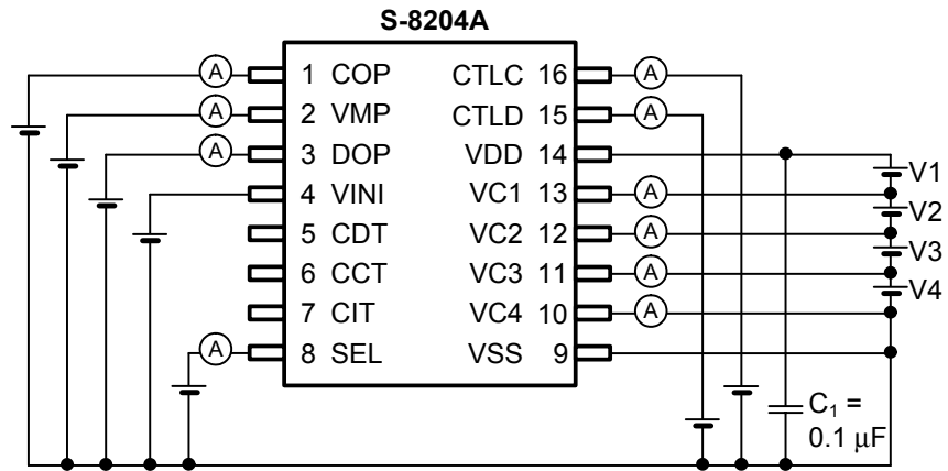
Figure 8 Test Circuit 5
