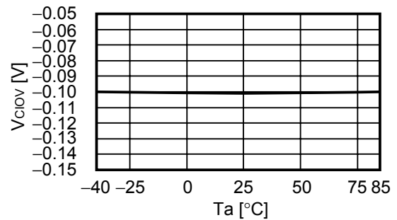
2.12 V_{CIOV} vs. T_a
