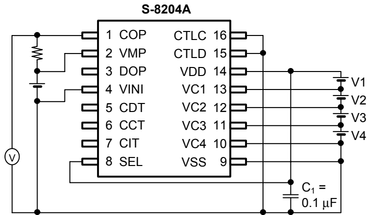
Figure 7 Test Circuit 4
