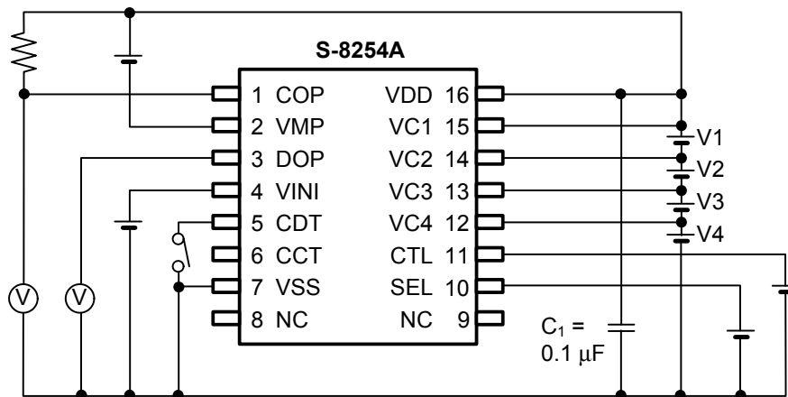
Figure 5 Test Circuit 2
