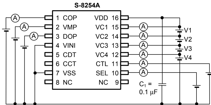
Figure 8 Test Circuit 5
