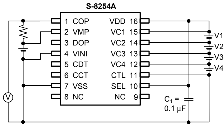
Figure 7 Test Circuit 4
