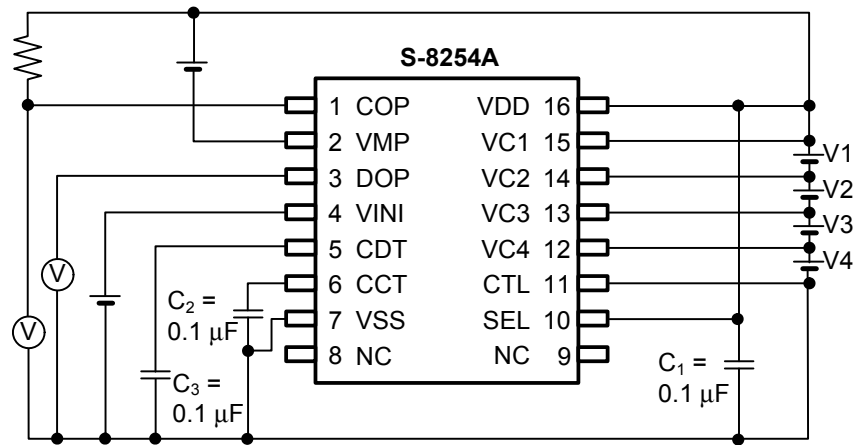
Figure 6 Test Circuit 3
