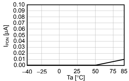
1.4 I_{PDN} vs. T_a
