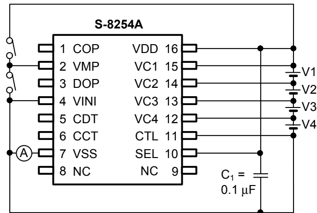
Figure 4 Test Circuit 1
