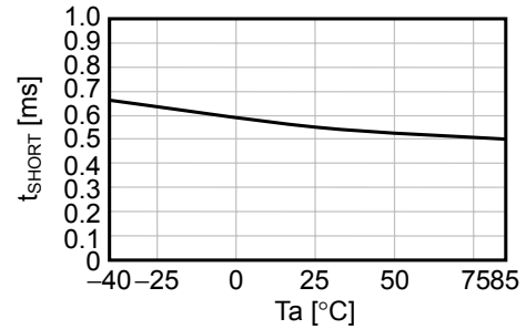
(12) t_{SHORT} vs. T_a
