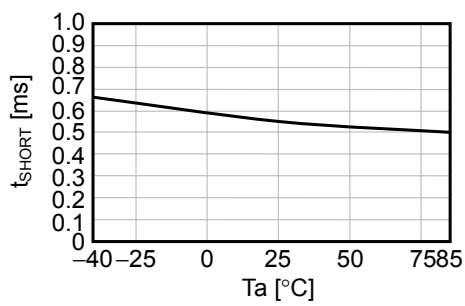
(15) t_{SHORT} vs. T_a
