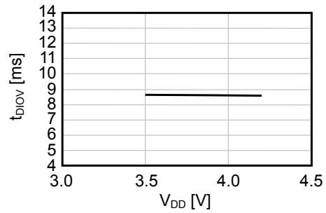
(8) t_{DIOV} vs. V_{DD}
