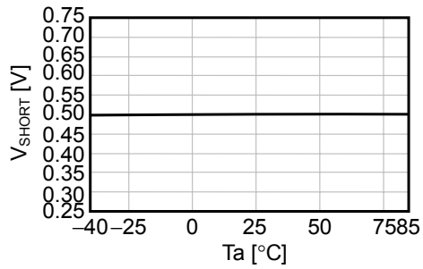
(13) V_{SHORT} vs. T_a
