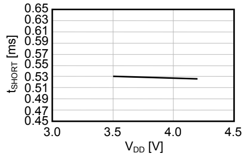
(14) t_{SHORT} vs. V_{DD}
