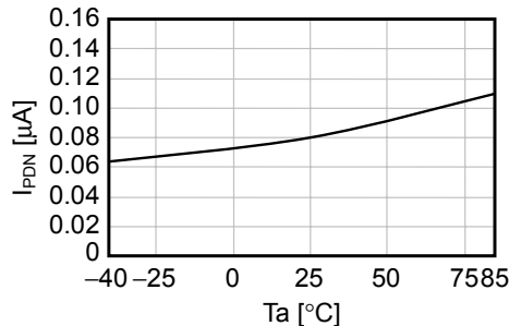
(2) I_{PDN} vs. T_a
