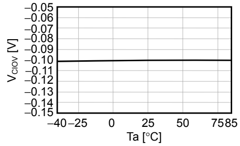
(10) V_{CIOV} vs. T_a
