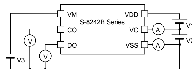
Figure 6 Test circuit 2
