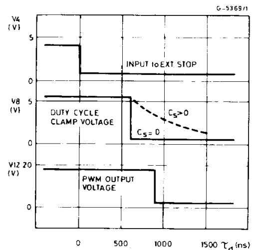
Figure 7 : Shutdown Timing.
