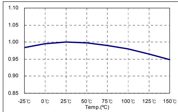
Figure 4. Operating Current
