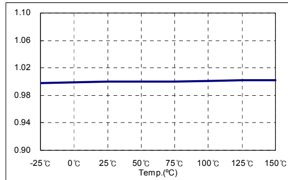
Figure 6. Maximum Duty
