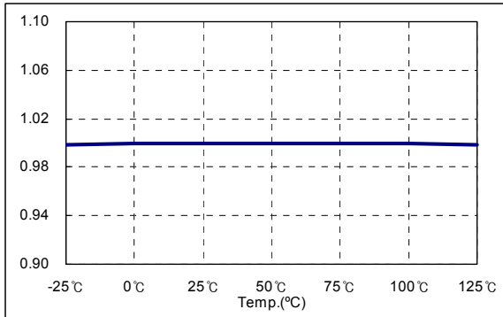
Figure 13. Burst Mode Low Threshold Voltage
