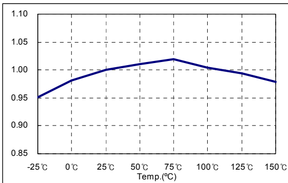
Figure 5. Initial Frequency
