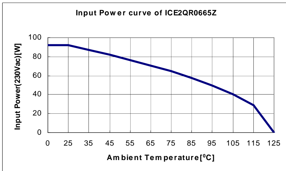
Figure 13 Input Power curve V_{in}=230V_{ac} ; P_{in}=f(T_a)
