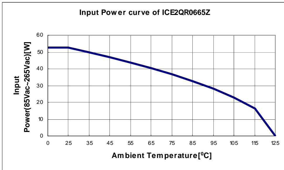
Figure 12 Input Power curve V_{in}=85\sim 265V_{ac} ; P_{in}=f(T_a)
