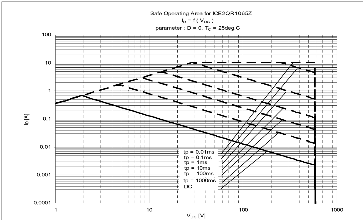
Figure 9 Safe Operating Area(SOA) curve for ICE2QR1065Z
