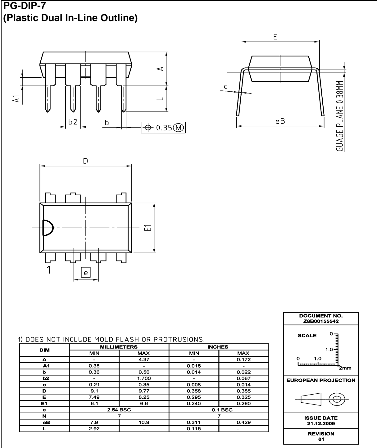
Figure 14 PG-DIP-7
