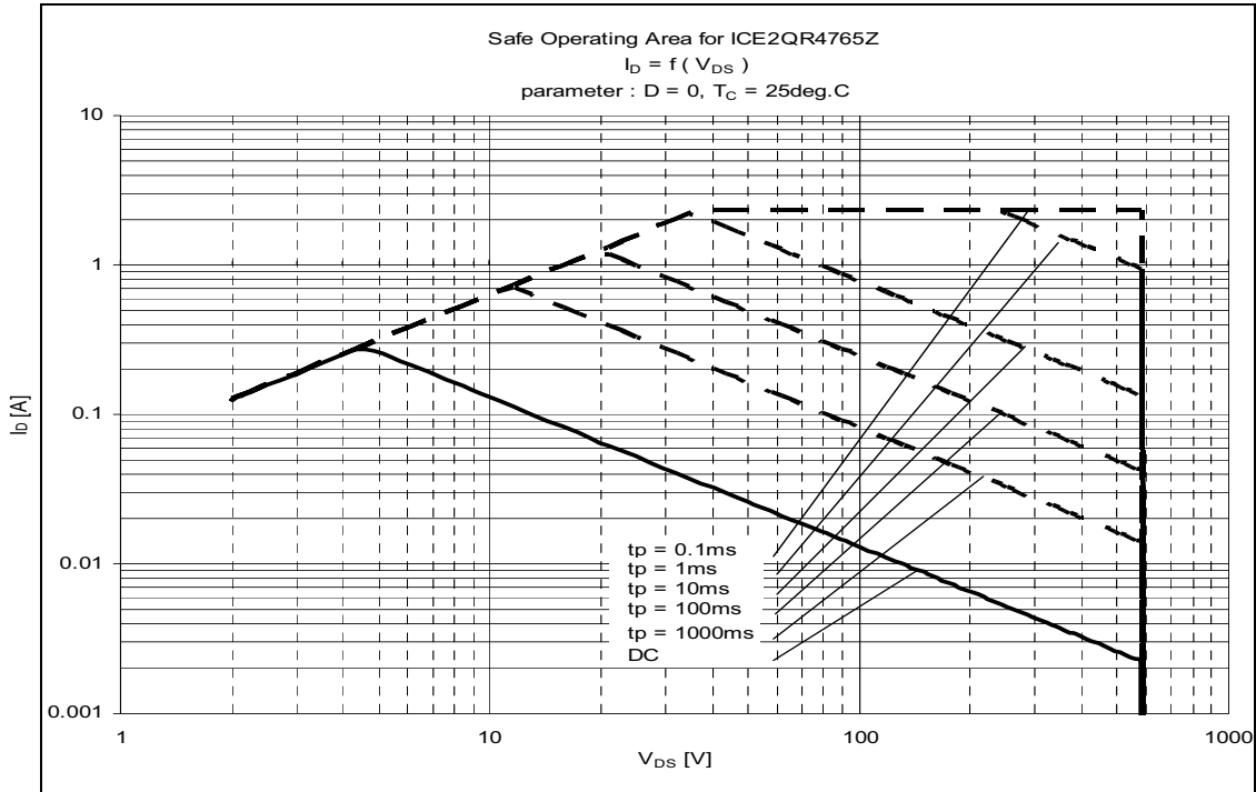
Figure 9 Safe Operating Area(SOA) curve for ICE2QR4765Z
