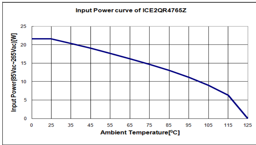
Figure 12 Input Power curve V_{in}=85\sim 265\text{Vac}; P_{in}=f(T_a)
