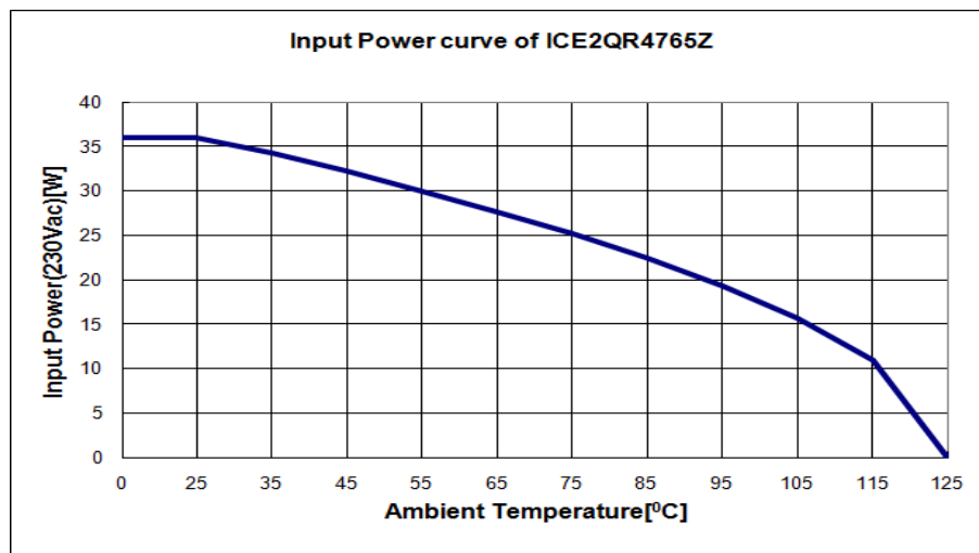
Figure 13 Input Power curve V_{in}=230\text{Vac}; P_{in}=f(T_a)
