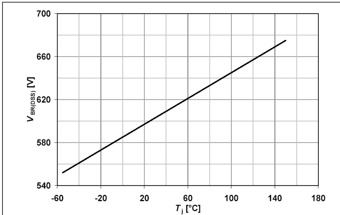
Figure 11 Drain-source breakdown voltage; V_{BR(DSS)}=f(T_j)
