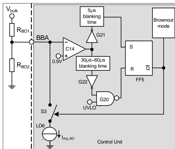
Figure 31 Brownout detection circuit
