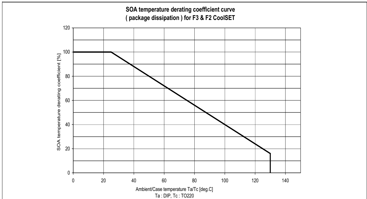
Figure 34 SOA temperature derating coefficient curve
