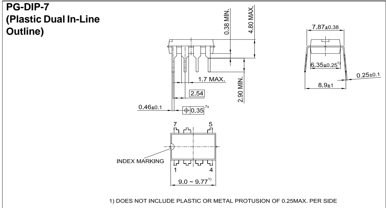
Figure 39 PG-DIP-7 (Pb-free lead plating Plastic Dual-in-Line Outline)
