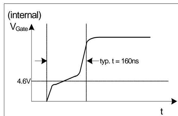
Figure 16 Gate Rising Slope
