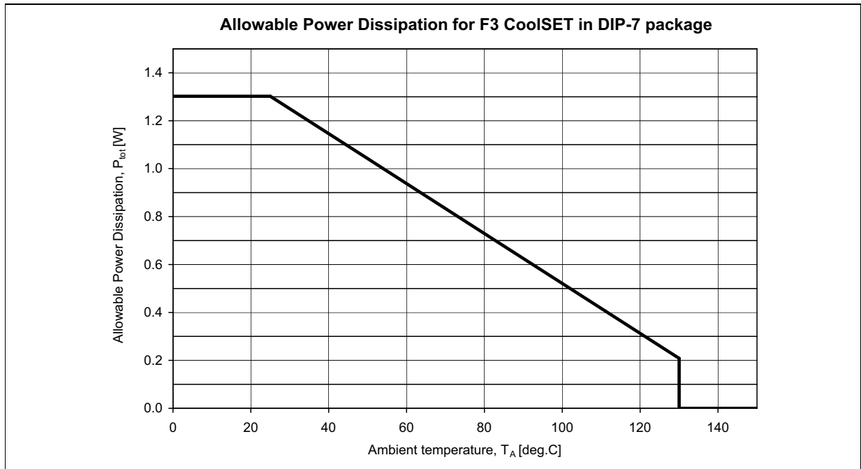
Figure 35 Power dissipation; P_{tot}=f(T_a)
