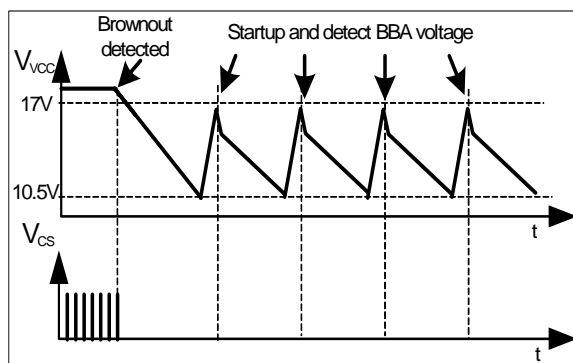
Figure 32 Brownout mode waveform
