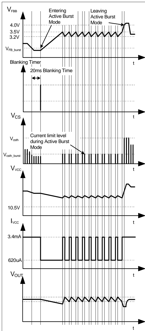
Figure 26 Signals in Active Burst Mode
