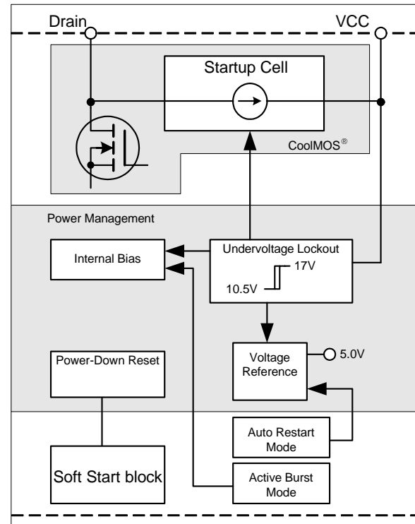
Figure 3 Power Management
