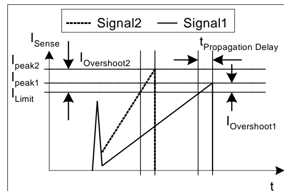
Figure 19 Current Limiting
