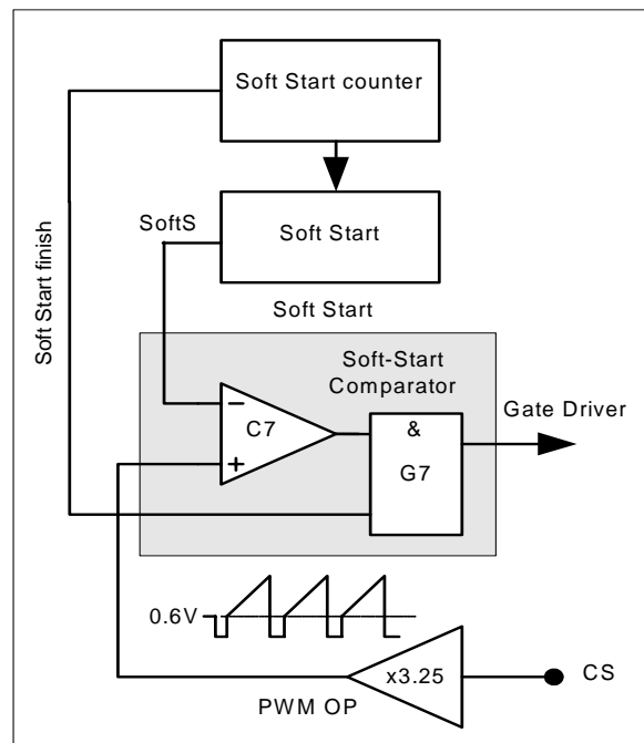
Figure 9 Soft Start
