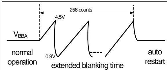
Figure 23 Waveform at extended blanking time
