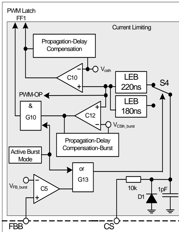
Figure 17 Current Limiting Block
