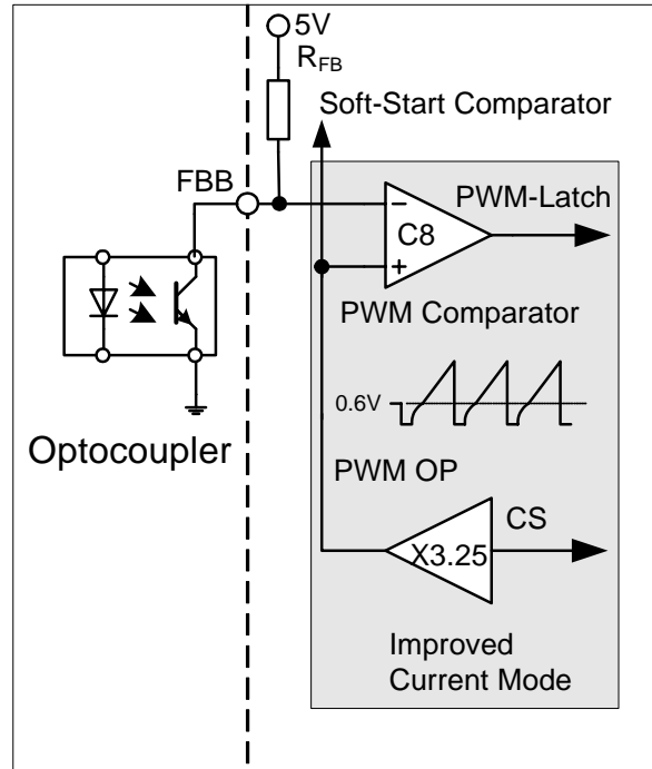
Figure 8 PWM Controlling
