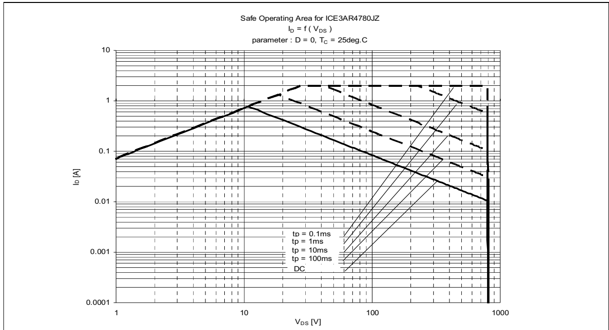
Figure 33 Safe Operating Area (SOA) curve for ICE3AR4780JZ
