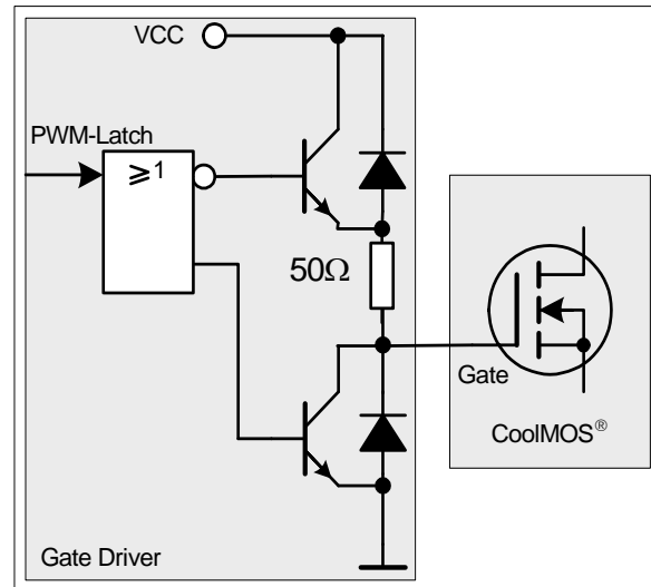
Figure 15 Gate Driver
