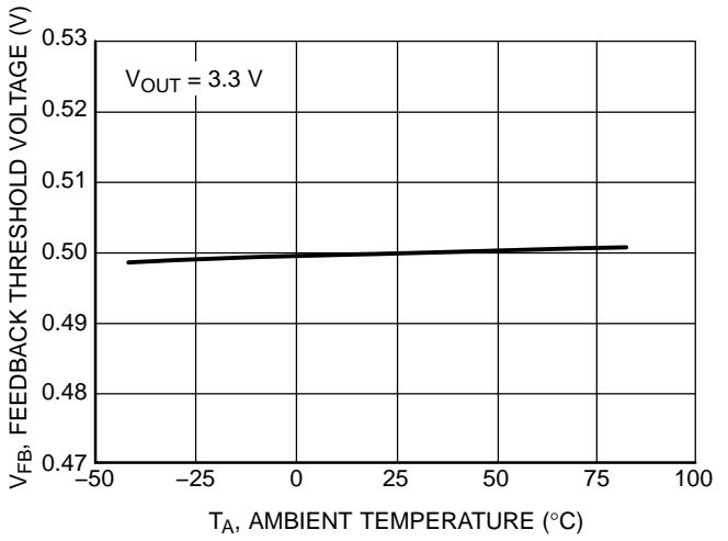
Figure 12. Feedback Threshold Voltage vs. Temperature
