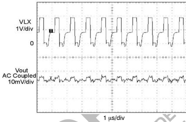
Figure 18. Light-Load PWM Switching Waveform ( V_{in} = 3.6\text{ V} , V_{out} = 1.5\text{ V} , I_{out} = 30\text{ mA} )
