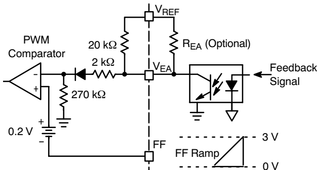
Figure 45. Optocoupler Driving V_{EA} Input
