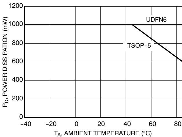
Figure 7. Power Derating
