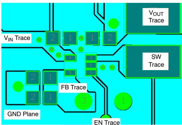
Figure 29. TSOP-5 Recommended Board Layout
