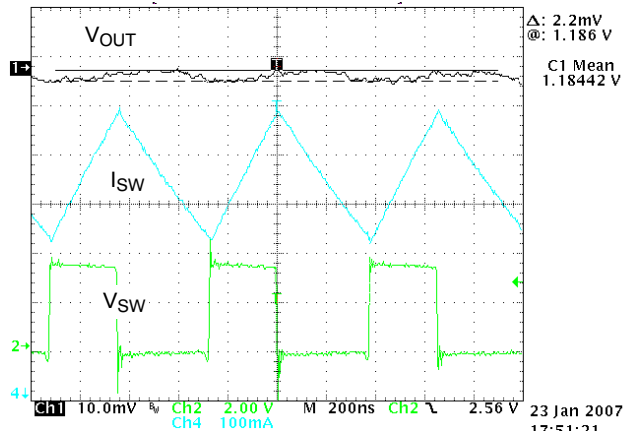
Figure 25. PWM Switching Waveforms (V_{IN} = 3.6\text{ V}, V_{OUT} = 1.2\text{ V}, I_{OUT} = 600\text{ mA}, Temperature = 25°C)
