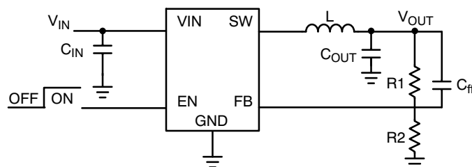
Figure 1. Typical Application
