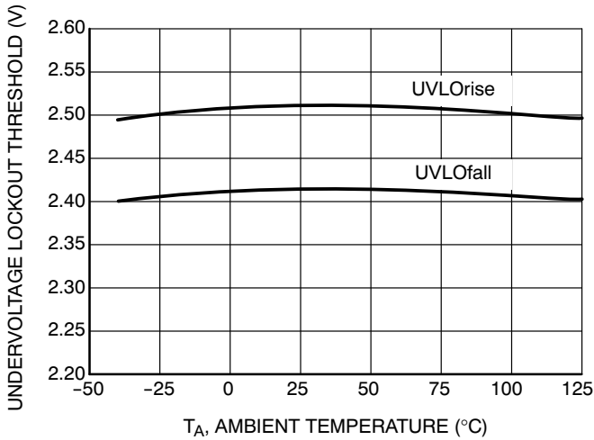
Figure 22. Undervoltage Lockout Threshold vs. Ambient Temperature
