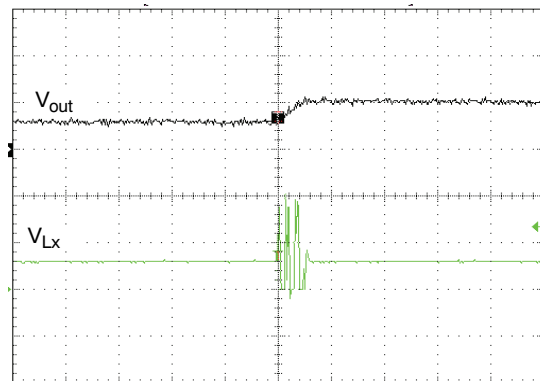
Figure 28. PFM Switching Waveforms ( V_{IN} = 3.6\text{ V} , V_{OUT} = 1.2\text{ V} , I_{OUT} = 0\text{ mA} , Temp = 25^\circ\text{C} )
