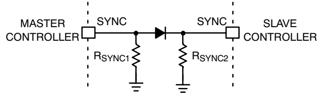
Figure 50. Master-Slave Configuration
