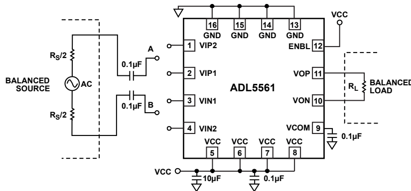
Figure 31. Basic Connections
