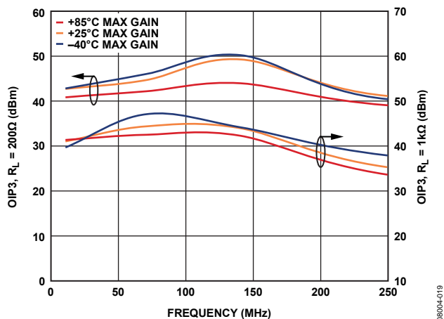
Figure 10. Output Third-Order Intercept vs. Frequency, Over Temperature, Output Level at 2 V p-p Composite, R_L = 200 \Omega and R_L = 1 k\Omega
