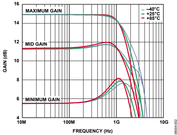
Figure 3. Gain vs. Frequency Response for 200 Ω Differential Load, Av = 6 dB, 12 dB, and 15.5 dB over Temperature
