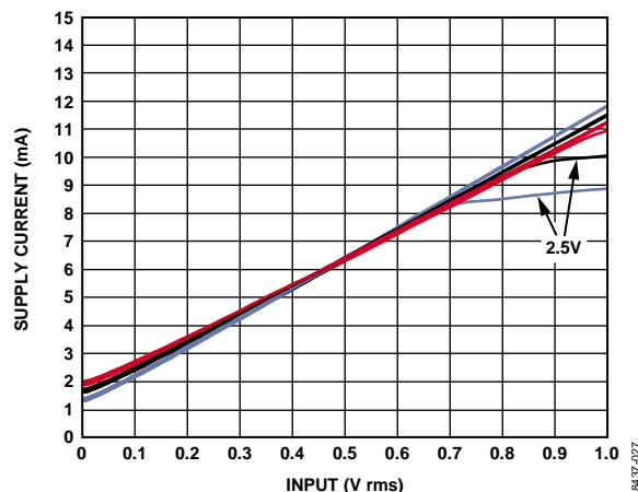
Figure 27. Supply Current vs. Input Level, 2.5 V, 3.0 V, and 3.3 V Supplies, 900 MHz Frequency, at -40°C, +25°C, and +85°C
