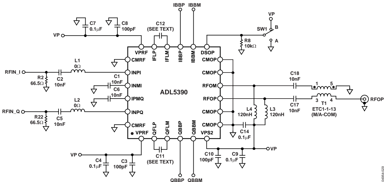
Figure 29. Basic Connections
