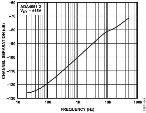
Figure 33. Channel Separation vs. Frequency
