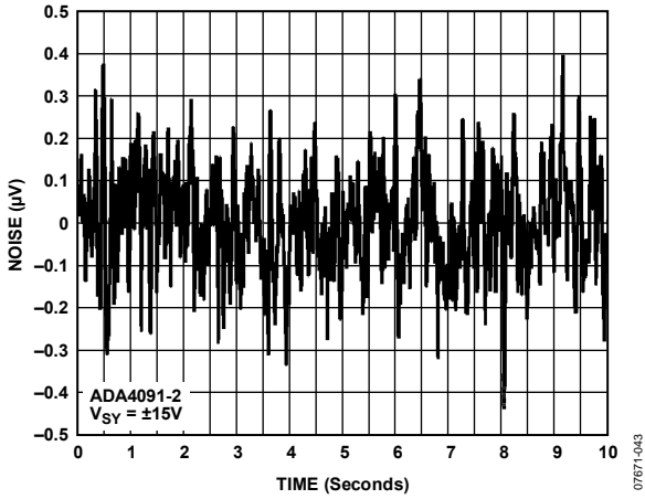
Figure 32. Voltage Noise, V_{p-p}
