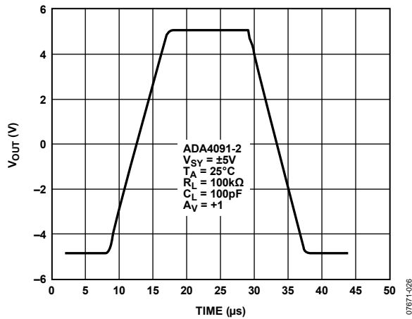
Figure 14. Large Signal Transient Response
