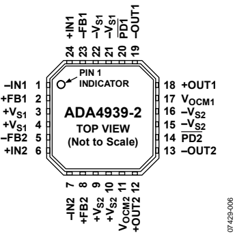
Figure 6. ADA4939-2 Pin Configuration
