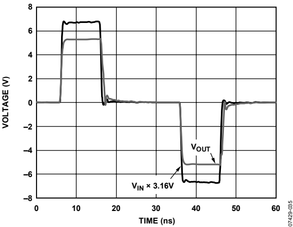
Figure 30. Overdrive Recovery, G = 3.16
