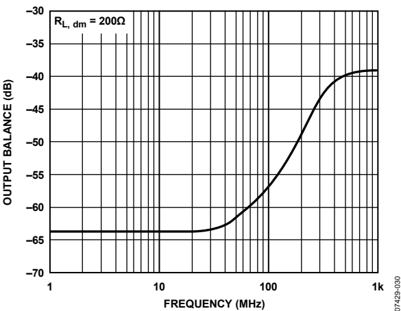
Figure 28. Output Balance vs. Frequency
