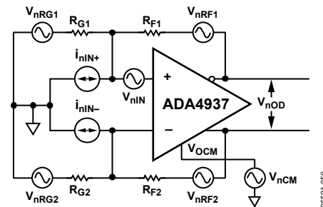
Figure 50. ADA4937 Noise Model
