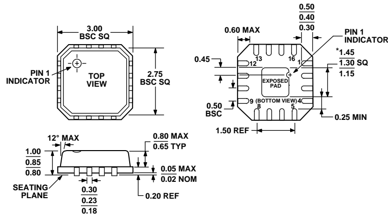
Figure 9. 16-Lead Lead Frame Chip Scale Package [LFCSP_VQ] 3 mm x 3 mm Body (CP-16-2) Dimensions shown in millimeters
