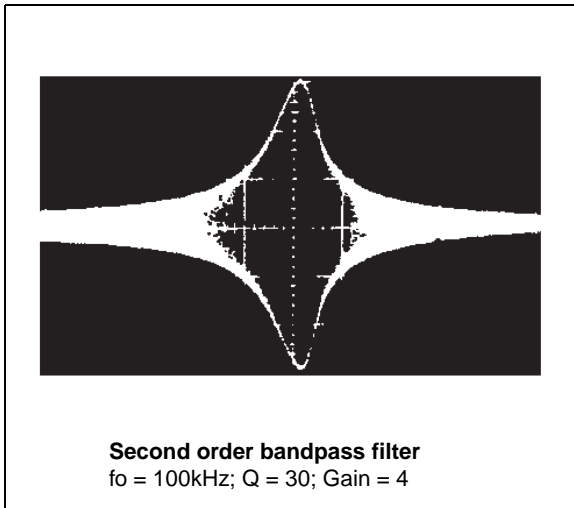
Figure 23. Output A
